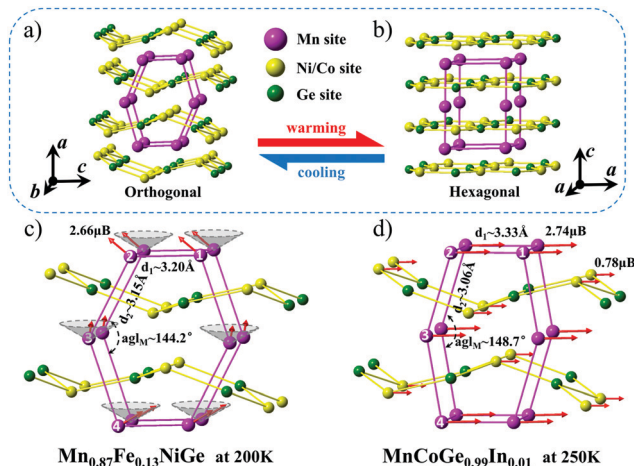
Fig. 1 (a and b) Sketches of orthorhombic and hexagonal structures of MnNiGe/MnCoGe, where the change of unit cell (magenta lines enclosed) and atomic chains can be clearly identified. (c and d) Fragments of the cone-spiral magnetic structure (Mn 0.87 Fe 0.13 NiGe) and linear FM (MnCoGe 0.99 In 0.01 ) structures viewed along the b axes with selected distances labeled in Å, the Mn1–Mn2 distance d 1 along the c -axis, the Mn2–Mn3 distance d 2 , and the angle agl M of the Mn2–Mn3–Mn4 atomic chain are indicated.
