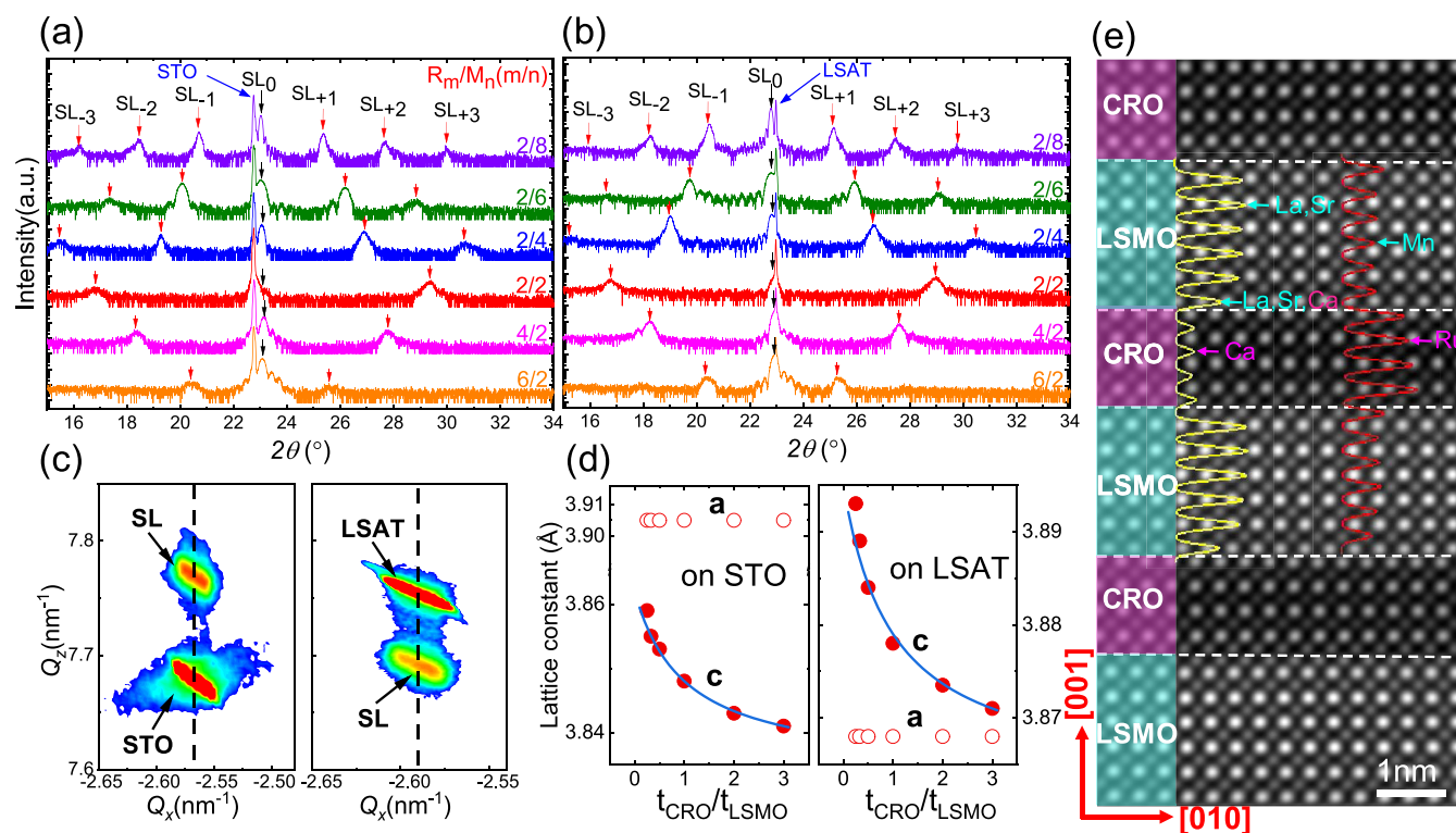
Figure 1. Structural characterization of CRO/LSMO SLs. (a) High-resolution \theta – 2\theta patterns of R_m/M_n SLs on STO and (b) LSAT. SL 0 represents the (001) main peak, while SL -1 , SL +1 , SL -2 , SL +2 , SL -3 , and SL +3 represent the satellite peaks. (c) RSM around the pseudocubic (103) reflection for the R_2/M_8 SLs on STO or LSAT substrate, respectively. (d) Out-of-plane and in-plane lattice constants as functions of the relative thickness of the CRO layer (defined as t_{\text{CRO}}/t_{\text{LSMO}} ) for the SLs on STO (left panel) or LSAT (right panel) substrates, deduced from the XRD and RSM results. The blue lines are the calculated out-of-plane lattice constants adopting the formula c_{\text{SL}} = (m \times c_{\text{CRO}} + n \times c_{\text{LSMO}})/(m + n) , where c_{\text{CRO}} and c_{\text{LSMO}} represent the c -axis lattice constants of CRO and LSMO sublayers. (e) High-angle annular dark-field (HAADF) image of the cross section of the R_4/M_6 SL, recorded along the [100] zone axis. The interface between CRO and LSMO is denoted by the dashed horizontal lines marked in white.
