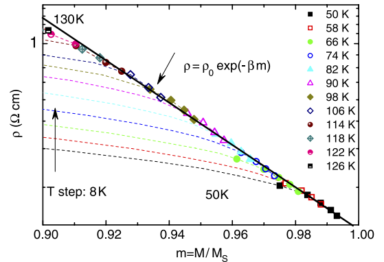
Figure 12. Resistivity as a function of normalized magnetization for the FM phase of LNCMO. Symbols and dashed lines denote the \rho - m curves of the FM state and the FM + PM/AFM state, respectively. Data collected at different temperatures are marked by different symbols. Solid lines are guides for the eyes.
